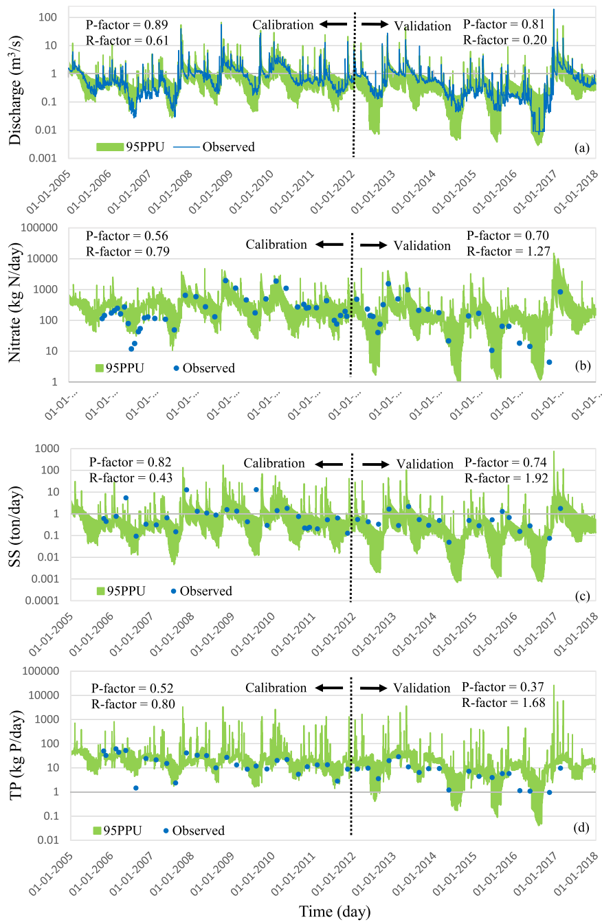
Fig. 4. Simulated and observed discharge (a), nitrate loads (b), suspended solids loads (c), and total phosphorus loads (d) at Montaverner Station. The difference between the lower and the upper bounds of the 95PPU demonstrates the necessity of quantifying and reporting the degree of uncertainty.
